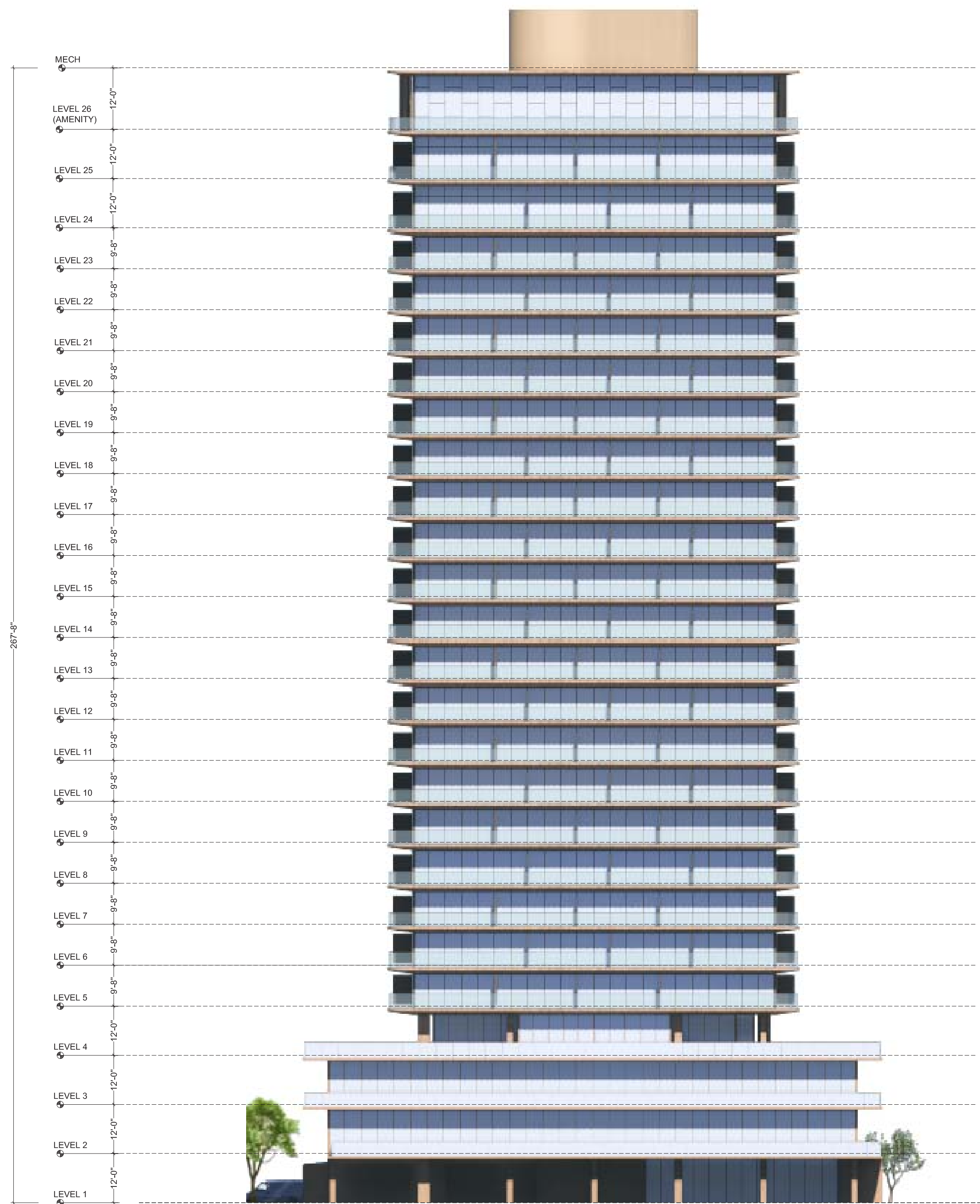
NORTH ELEVATION
