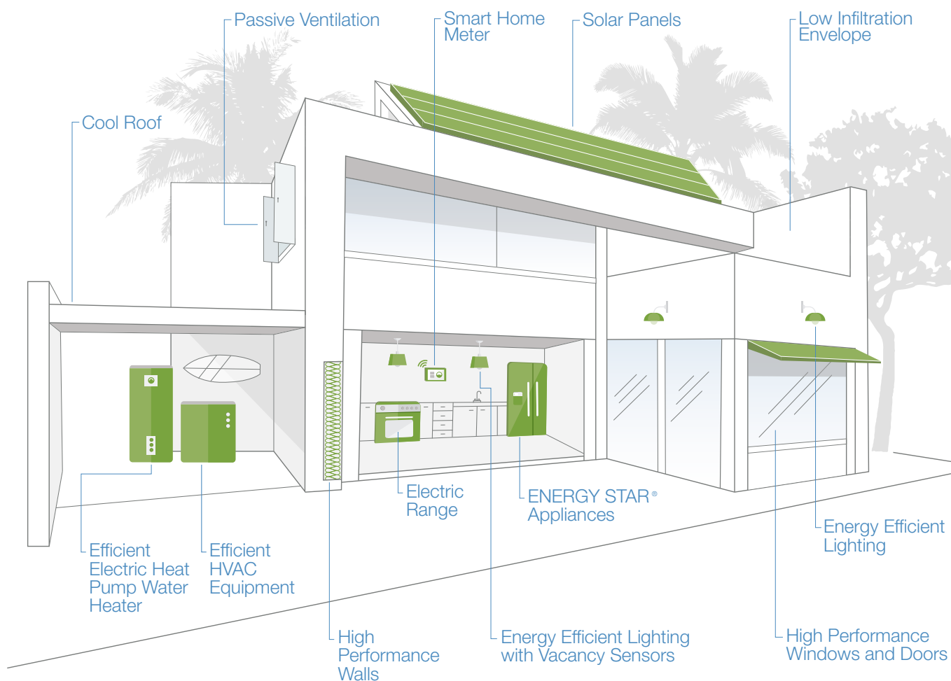
Figure 1. Zero net energy home energy efficiency and energy production features.
