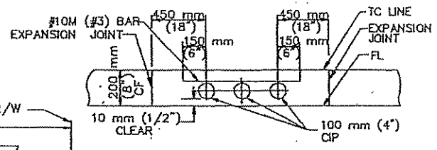
NOTE: APPLIES TO ANY NUMBER OF PIPES CURB PROFILE 200 mm (8") CURB FACE
