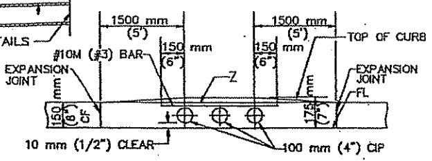
NOTE: APPLIES TO ANY NUMBER OF PIPES Z = TOP-OF-CURB LINE SHOWN ON PROFILE CURB PROFILE 150 mm (6") CURB FACE
