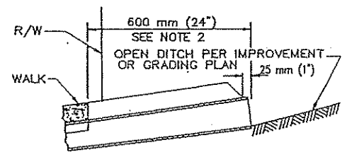
CASE III INLET GRADED DITCH SECTION
