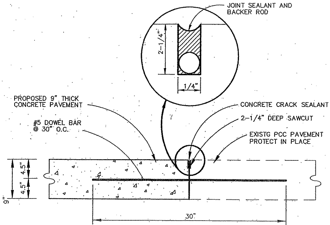
P.C.C. CONSTRUCTION JOINT N.T.S.
