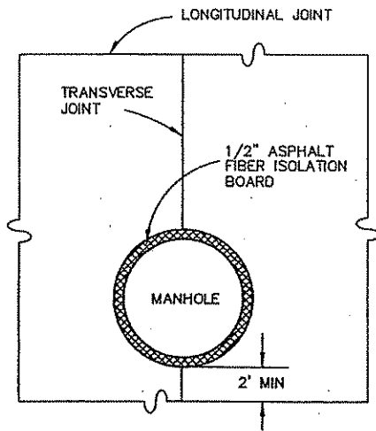
TYPICAL MANHOLE COVER JOINT DETAIL "A"
