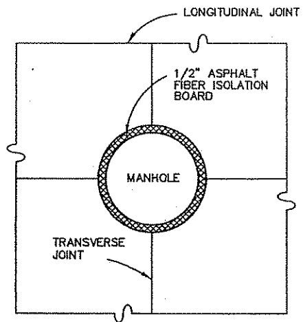
TYPICAL MANHOLE COVER JOINT DETAIL "B"
